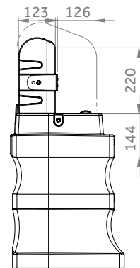
FUSE MOUNTING AREA MAXIMUM CAPACITY 6x FUSES
